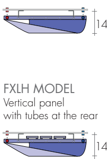
FXH MODEL Vertical panel
